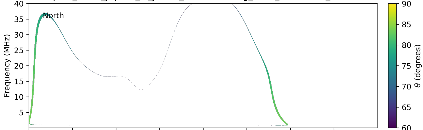
expres_earth_jupiter_io_jrm33_lossc-wid1deg_3kev_19941125_v11.cdf
