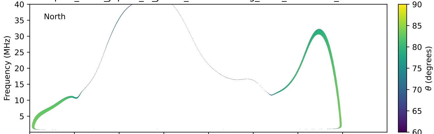
expres_earth_jupiter_io_jrm33_lossc-wid1deg_3kev_19941109_v11.cdf
