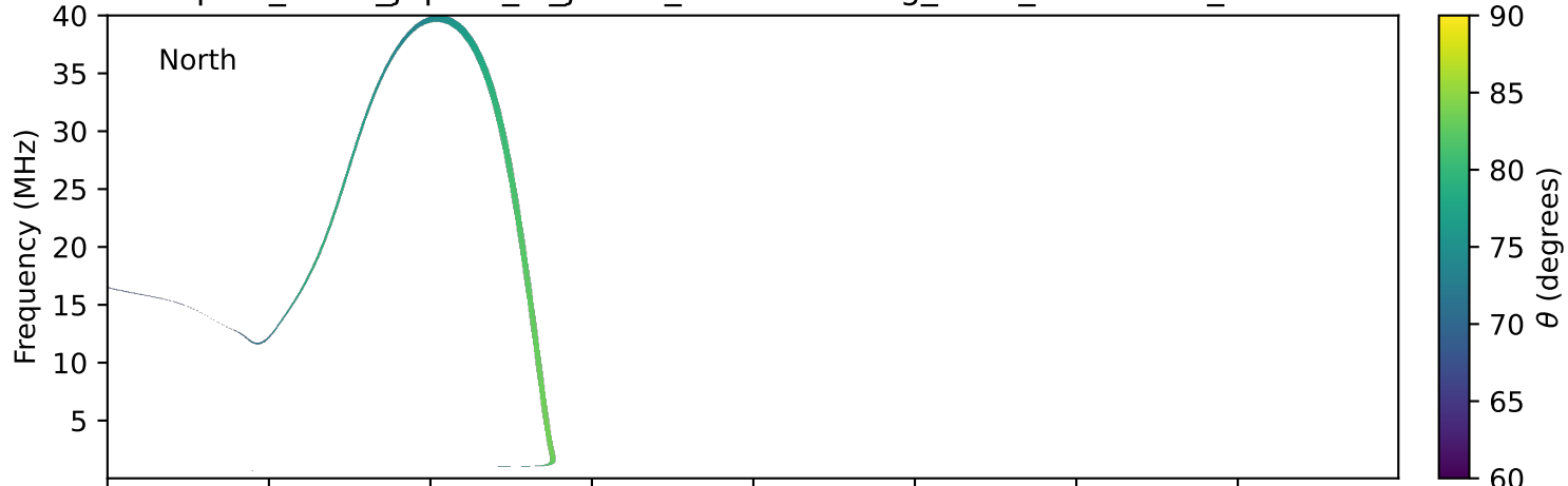
expres_earth_jupiter_io_jrm09_lossc-wid1deg_3kev_19941129_v11.cdf
