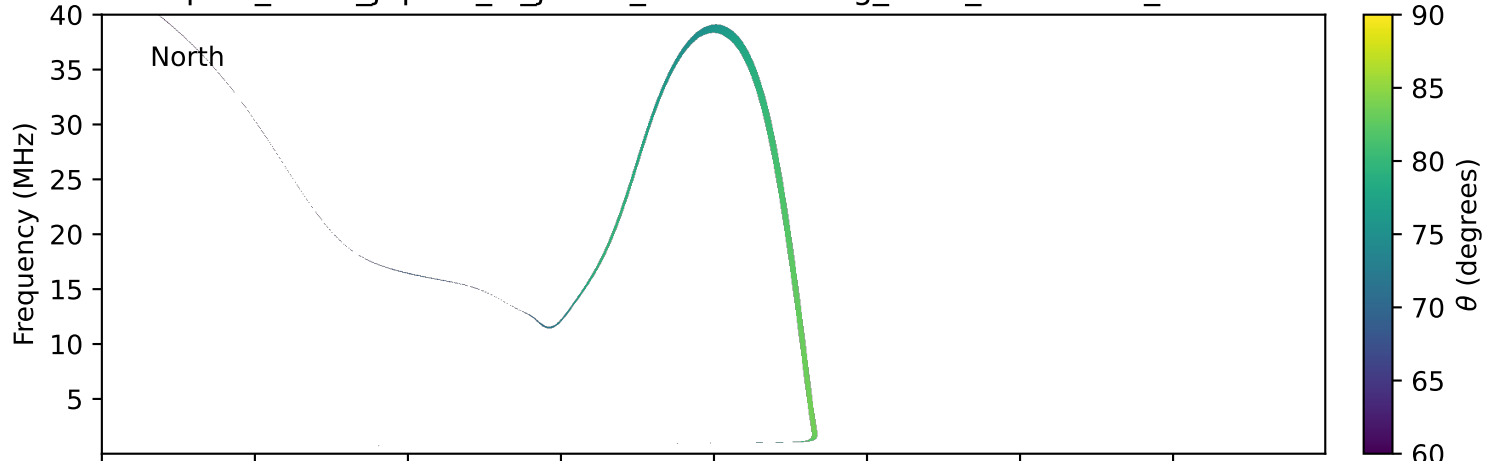
expres_earth_jupiter_io_jrm09_lossc-wid1deg_3kev_19941118_v11.cdf
