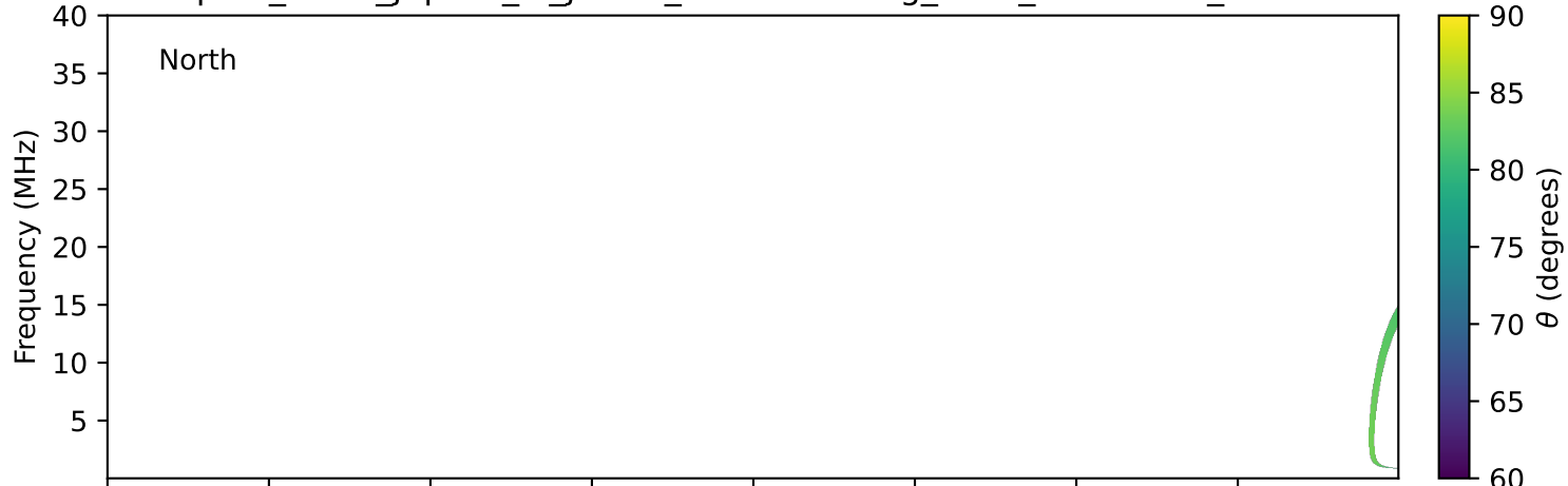
expres_earth_jupiter_io_jrm09_lossc-wid1deg_3kev_19941115_v11.cdf
