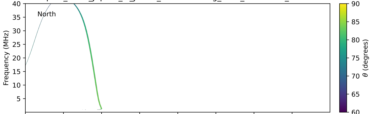
expres_earth_jupiter_io_jrm09_lossc-wid1deg_3kev_19941113_v11.cdf
