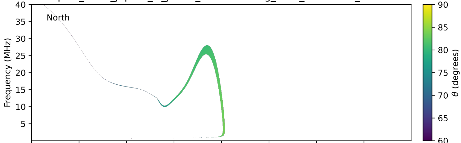
expres_earth_jupiter_io_jrm09_lossc-wid1deg_3kev_19941111_v11.cdf
