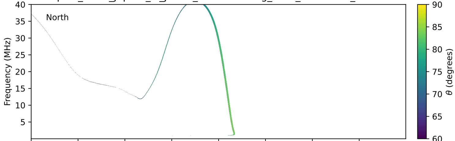
expres_earth_jupiter_io_jrm09_lossc-wid1deg_3kev_19941104_v11.cdf
