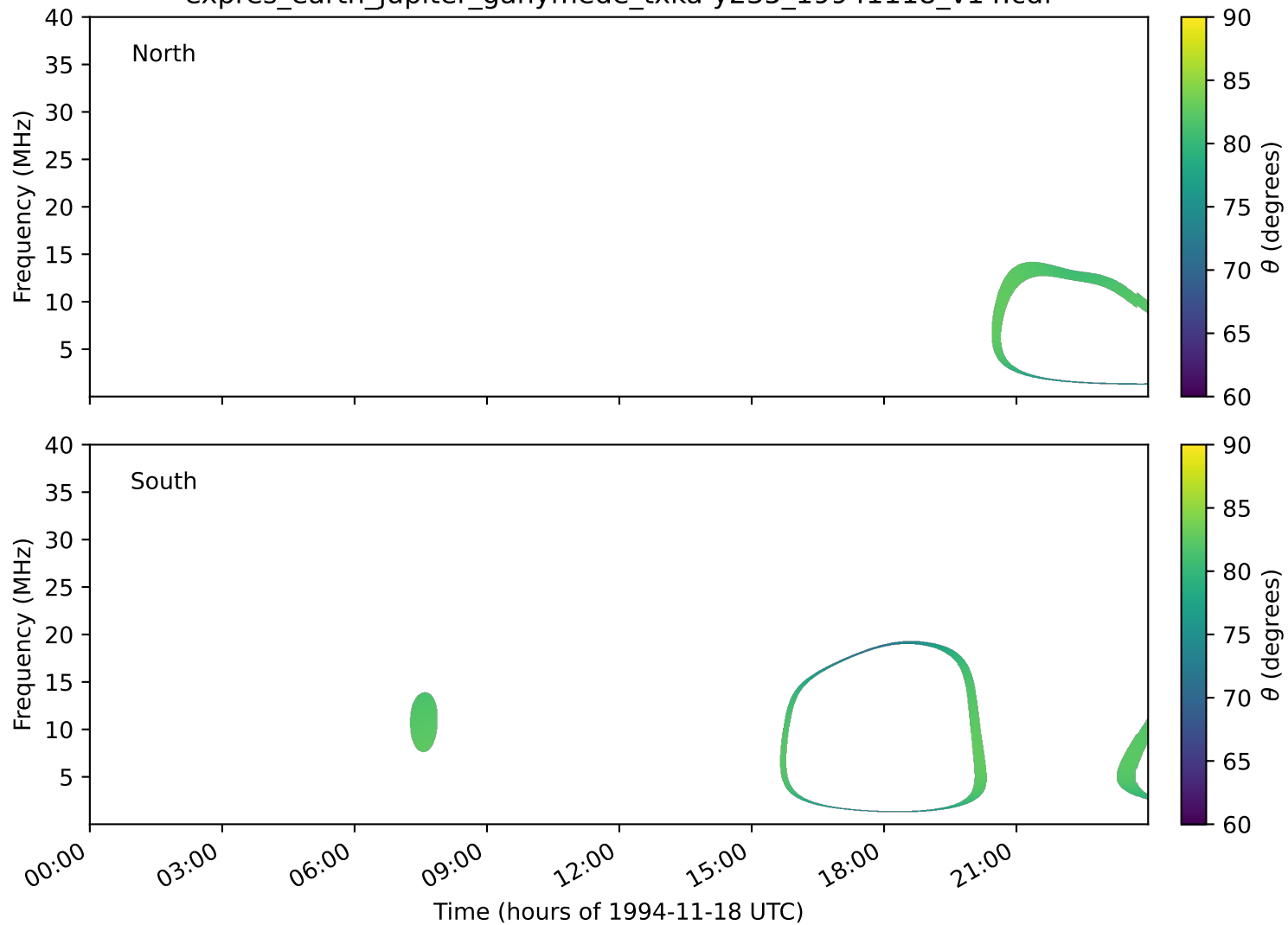
expres_earth_jupiter_ganymede_txka-y235_19941118_v14.cdf
