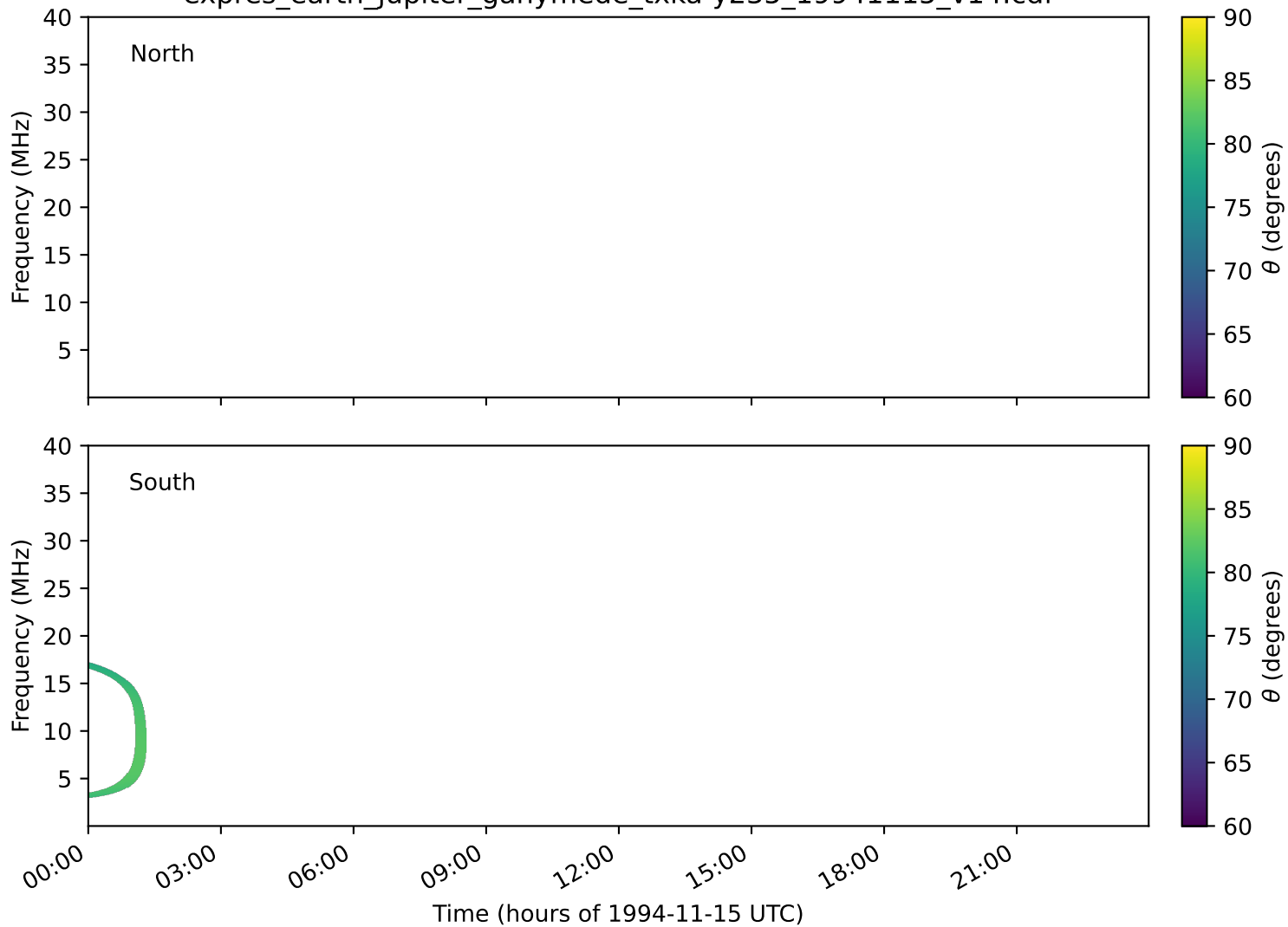
expres_earth_jupiter_ganymede_txka-y235_19941115_v14.cdf
