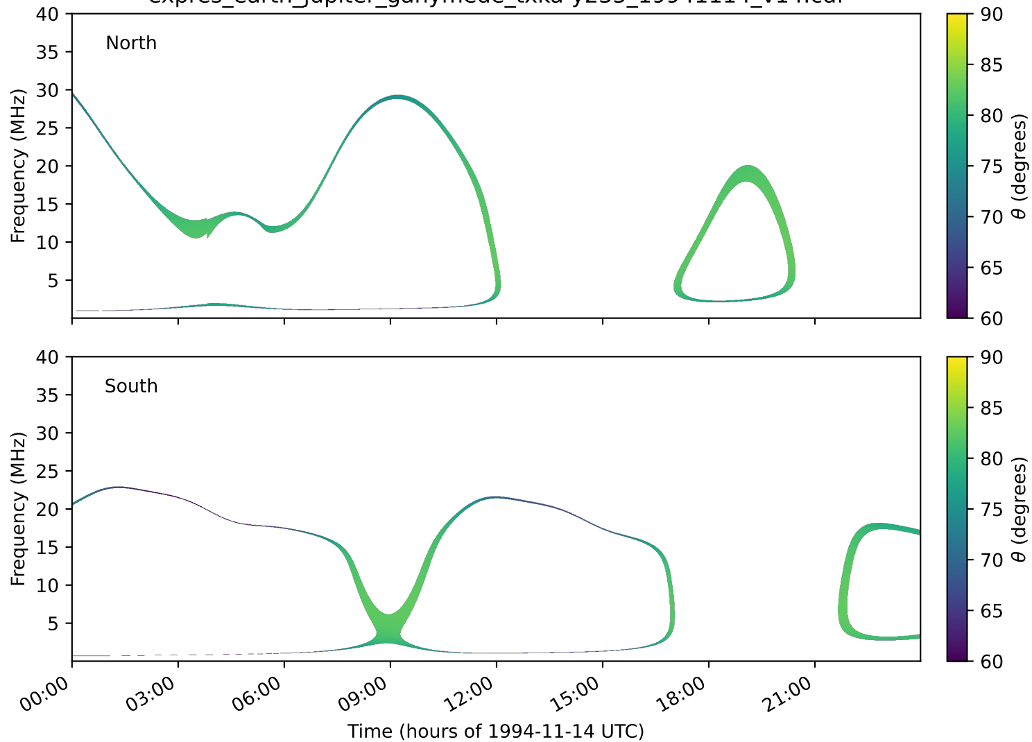
expres_earth_jupiter_ganymede_txka-y235_19941114_v14.cdf
