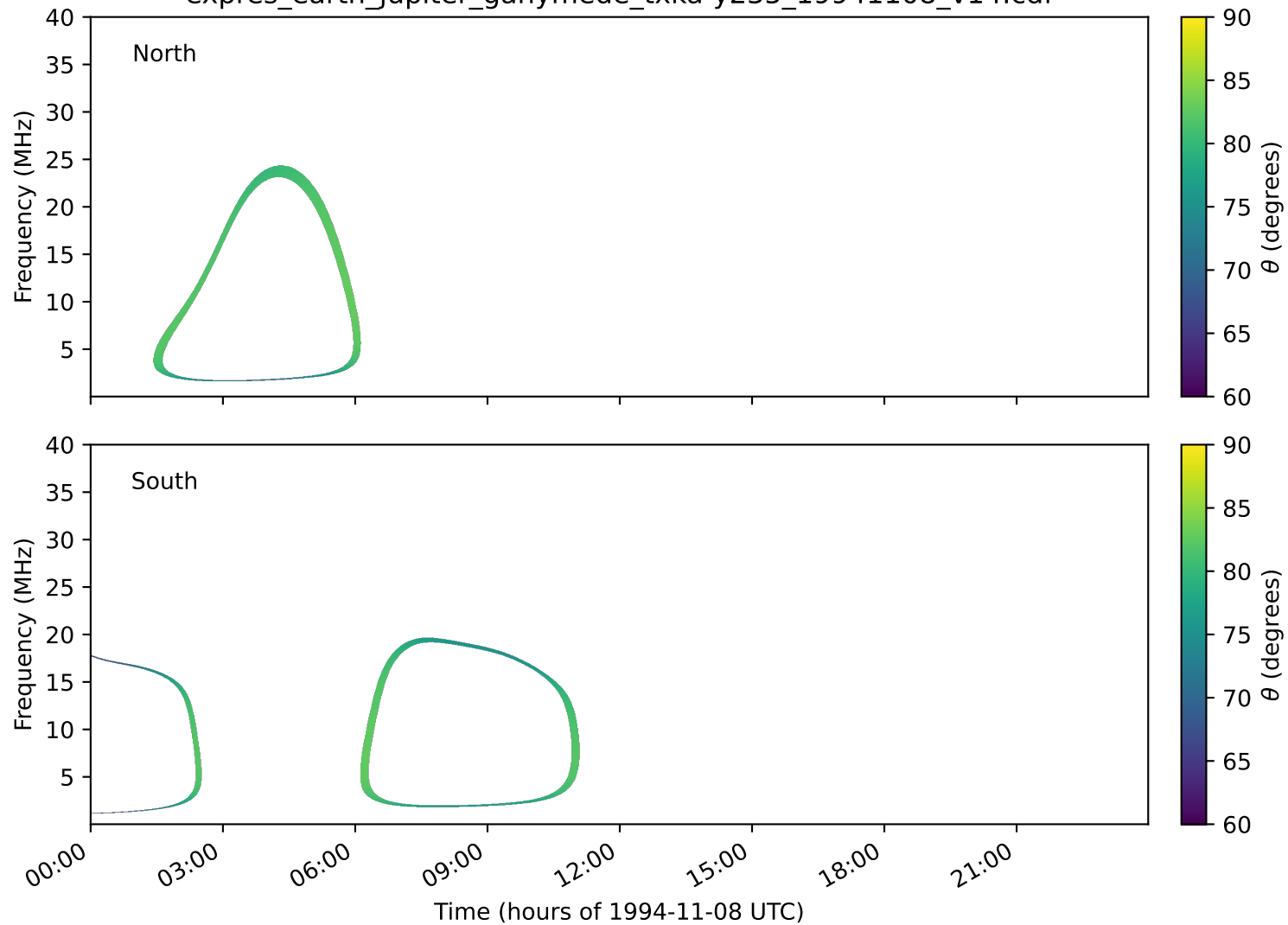
expres_earth_jupiter_ganymede_txka-y235_19941108_v14.cdf
