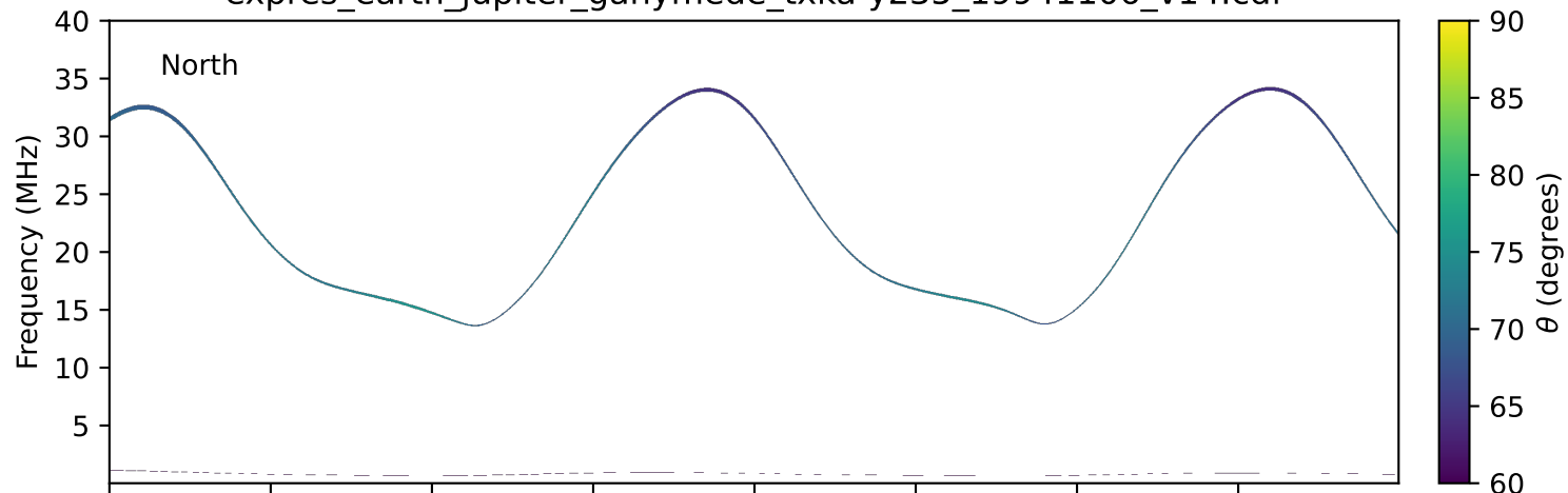
expres_earth_jupiter_ganymede_txka-y235_19941106_v14.cdf
