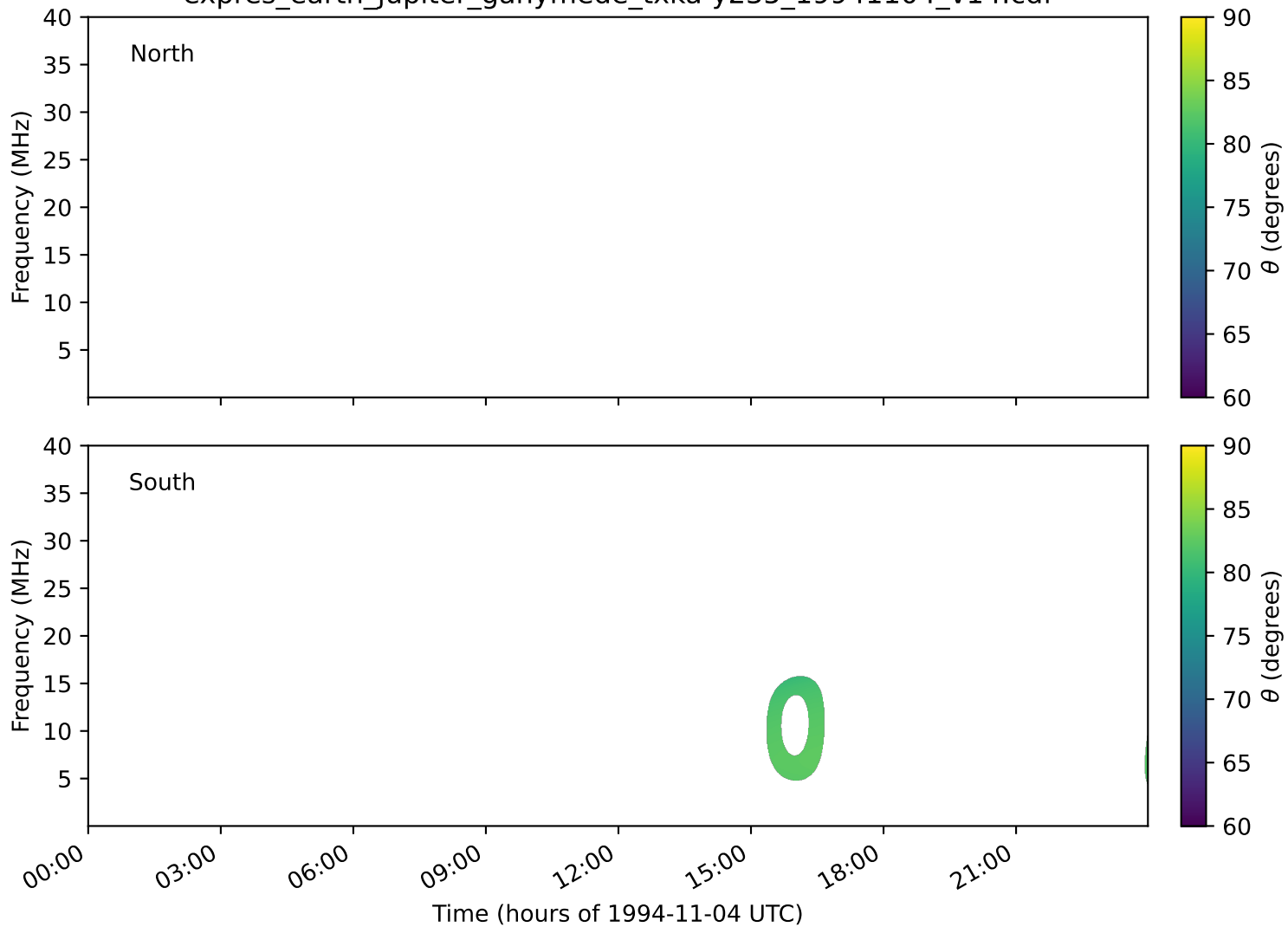
expres_earth_jupiter_ganymede_txka-y235_19941104_v14.cdf
