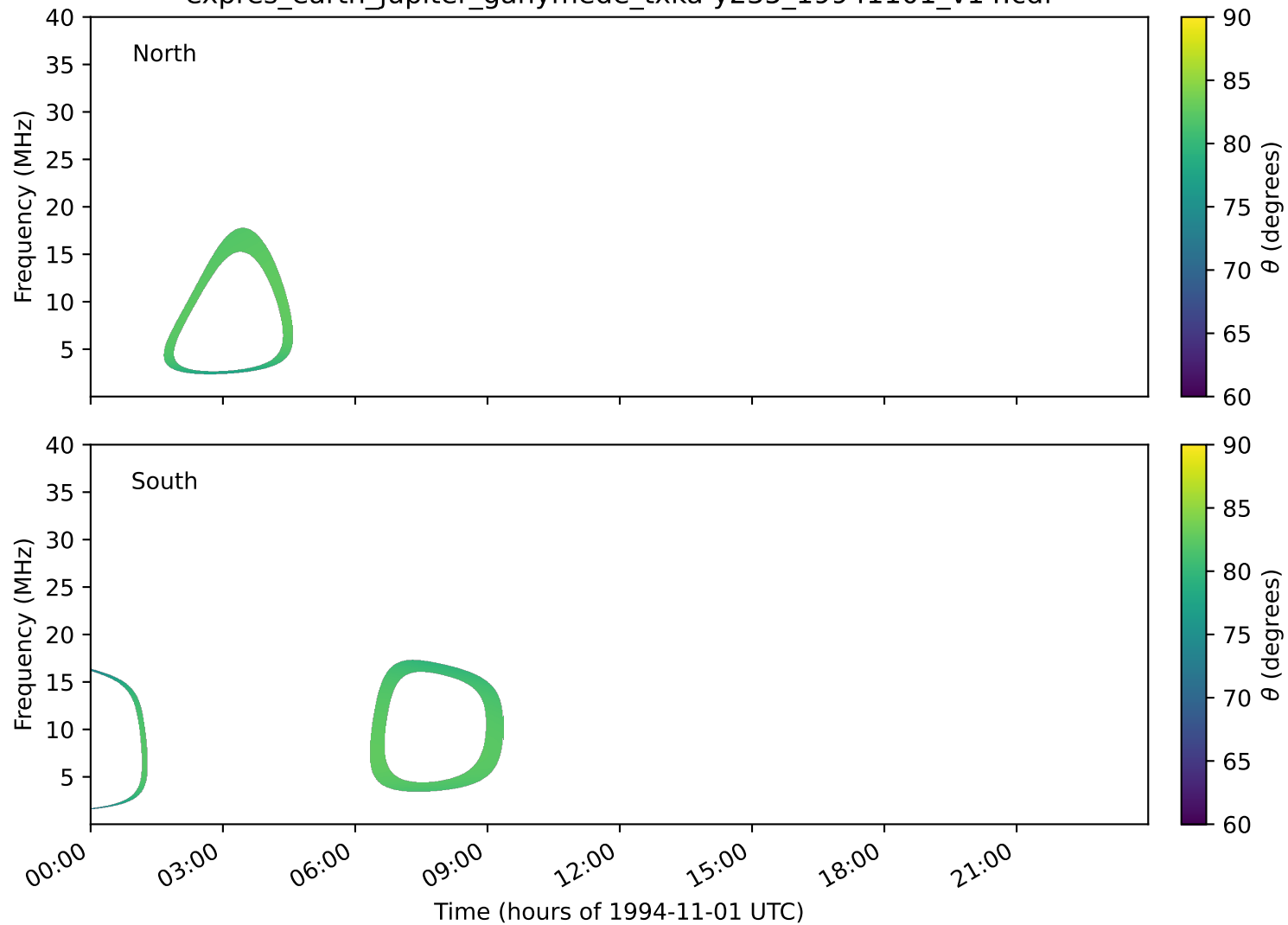
expres_earth_jupiter_ganymede_txka-y235_19941101_v14.cdf
