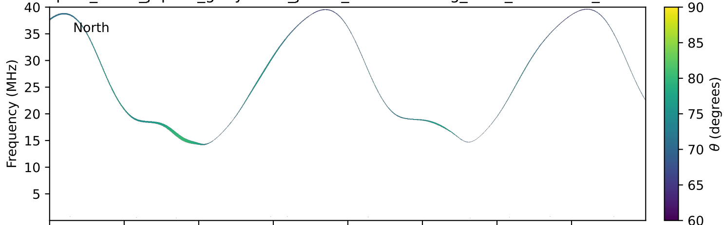
expres_earth_jupiter_ganymede_jrm33_lossc-wid1deg_3kev_19941106_v11.cdf
