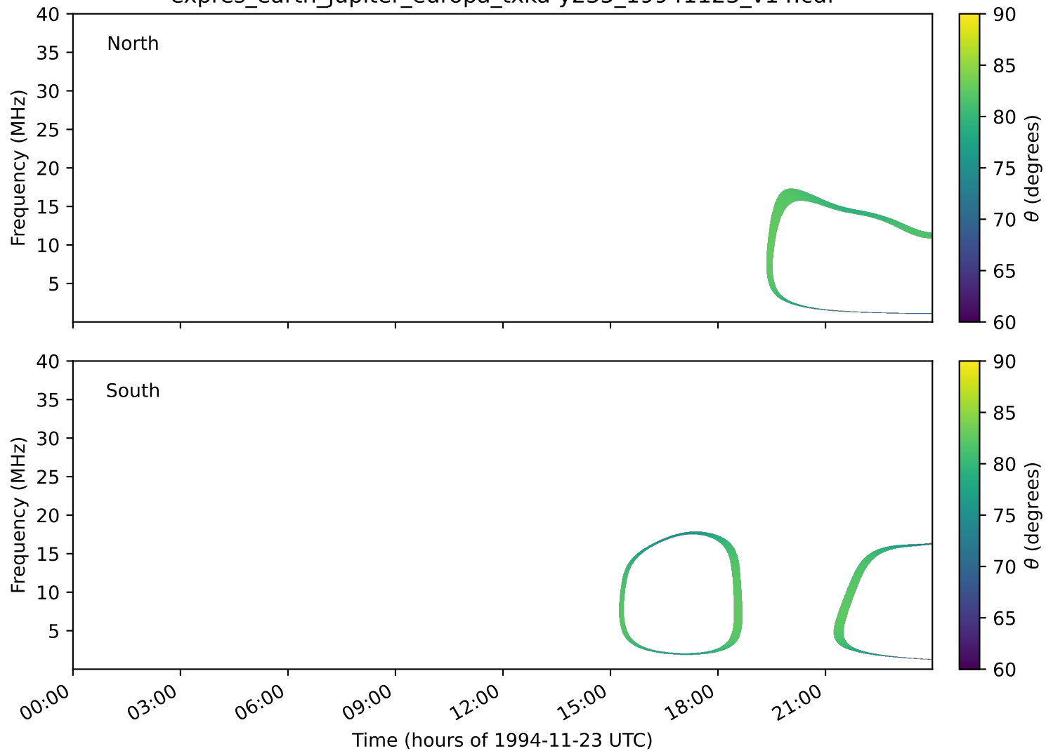
expres_earth_jupiter_europa_txka-y235_19941123_v14.cdf
