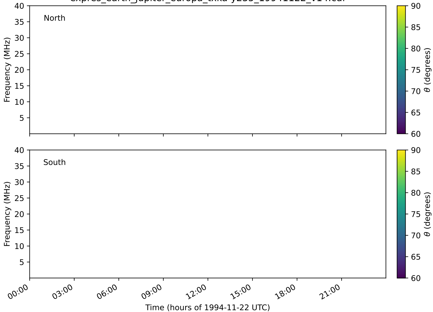
expres_earth_jupiter_europa_txka-y235_19941122_v14.cdf
