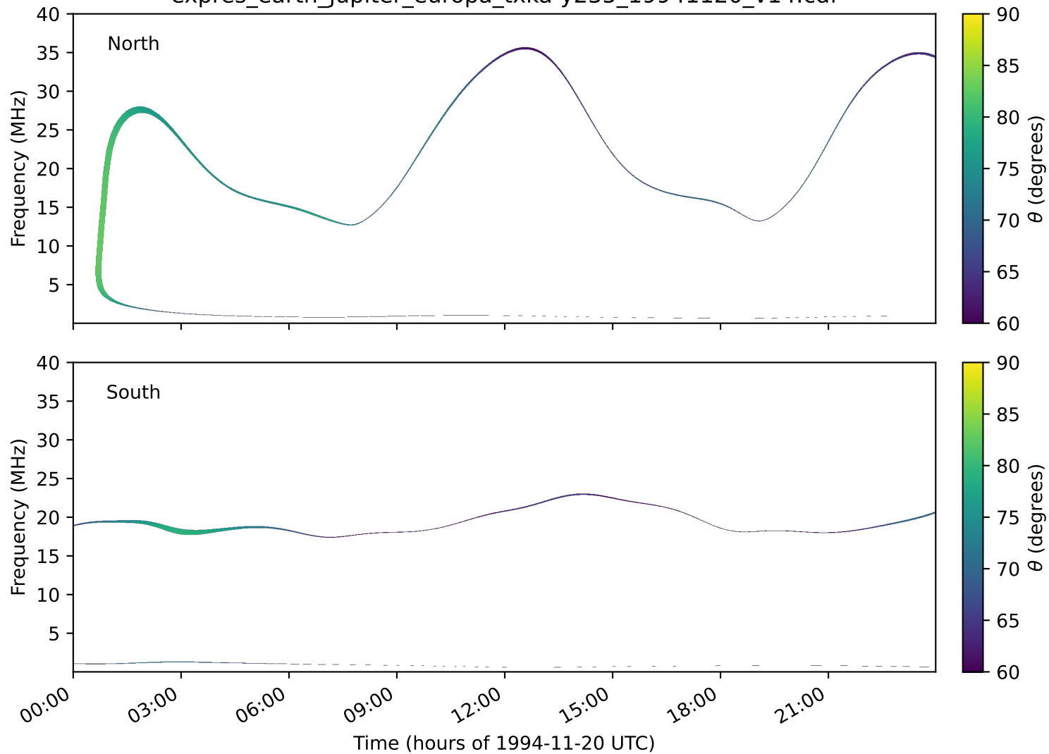
expres_earth_jupiter_europa_txka-y235_19941120_v14.cdf
