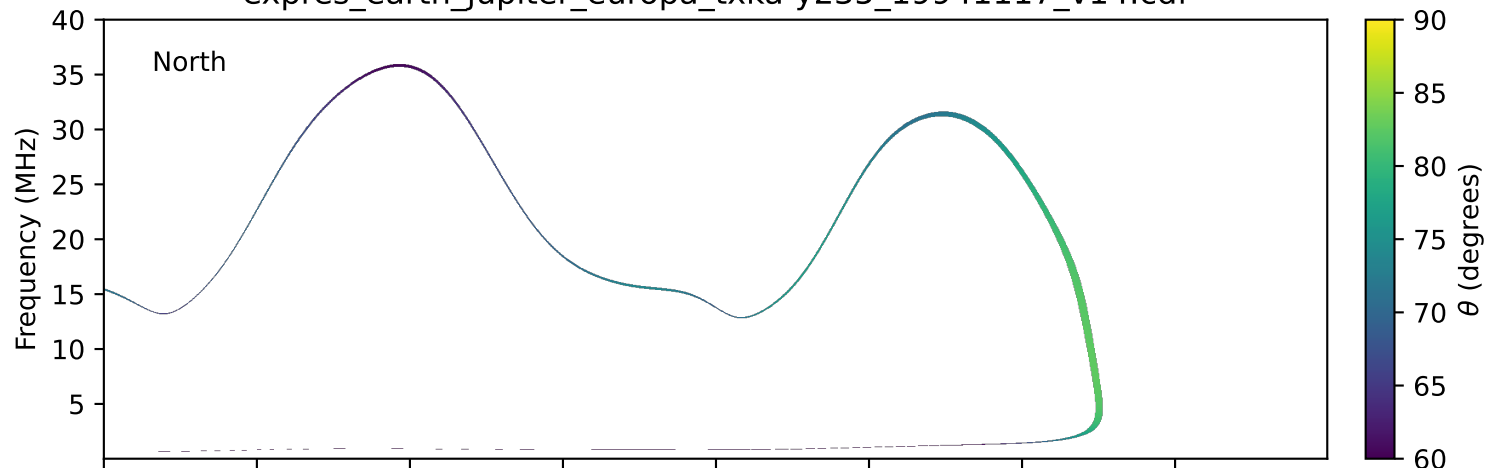
expres_earth_jupiter_europa_txka-y235_19941117_v14.cdf
