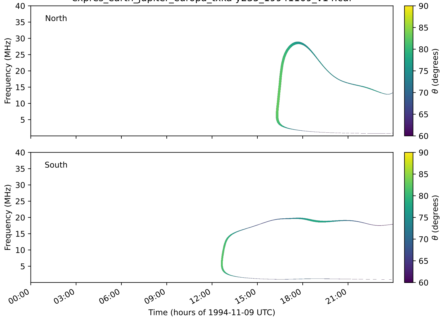
expres_earth_jupiter_europa_txka-y235_19941109_v14.cdf
