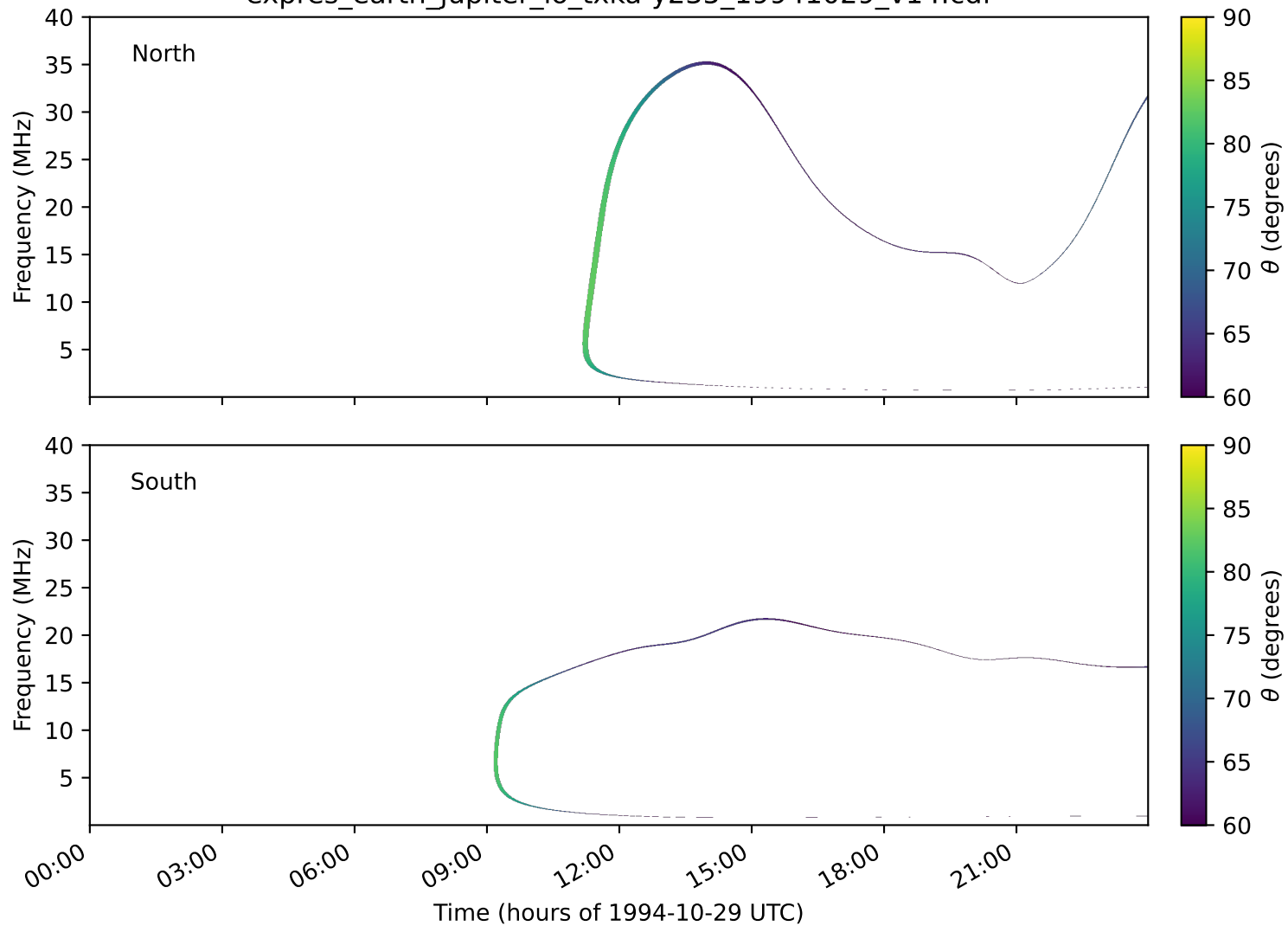
expres_earth_jupiter_io_txka-y235_19941029_v14.cdf
