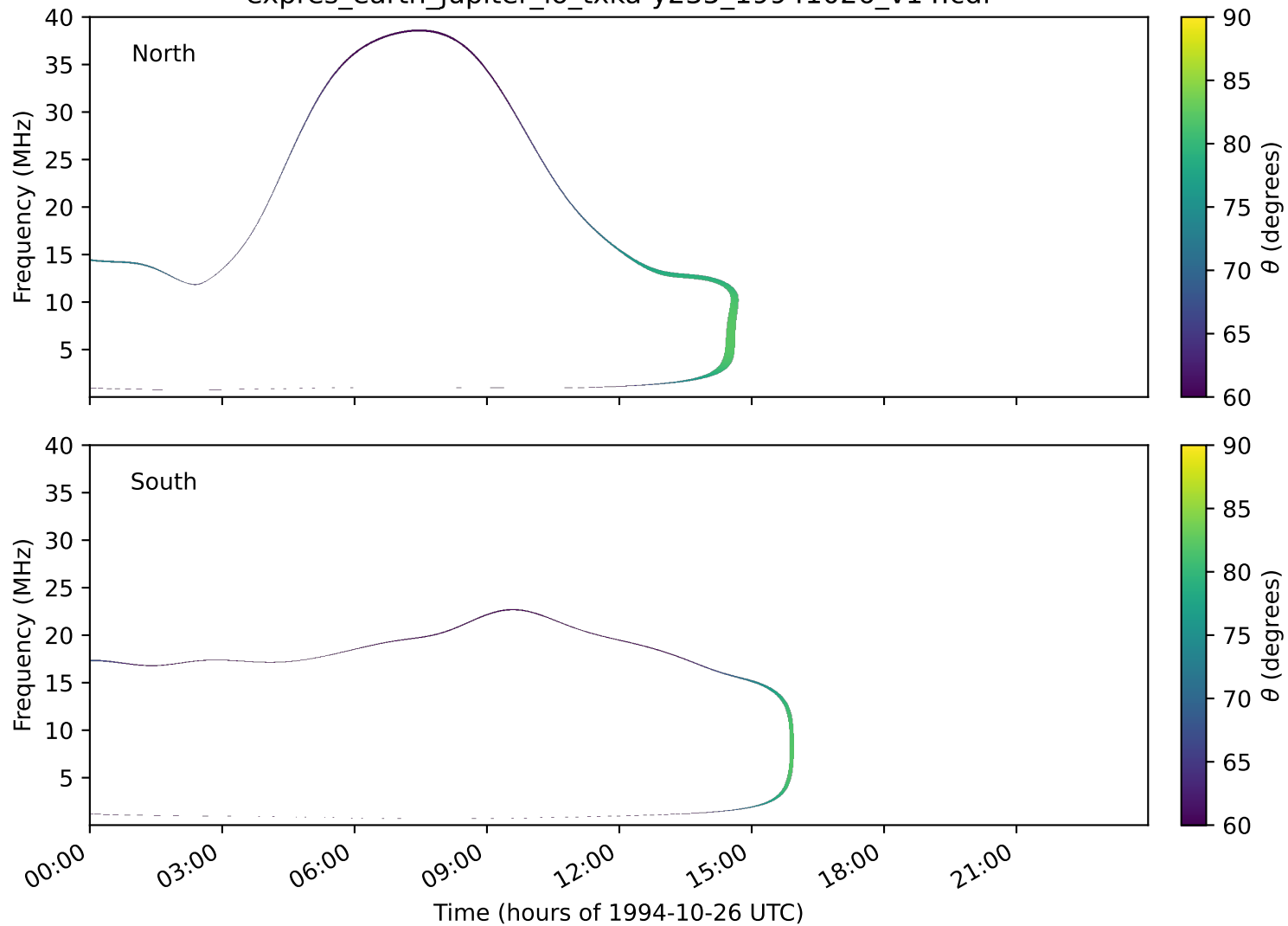
expres_earth_jupiter_io_txka-y235_19941026_v14.cdf
