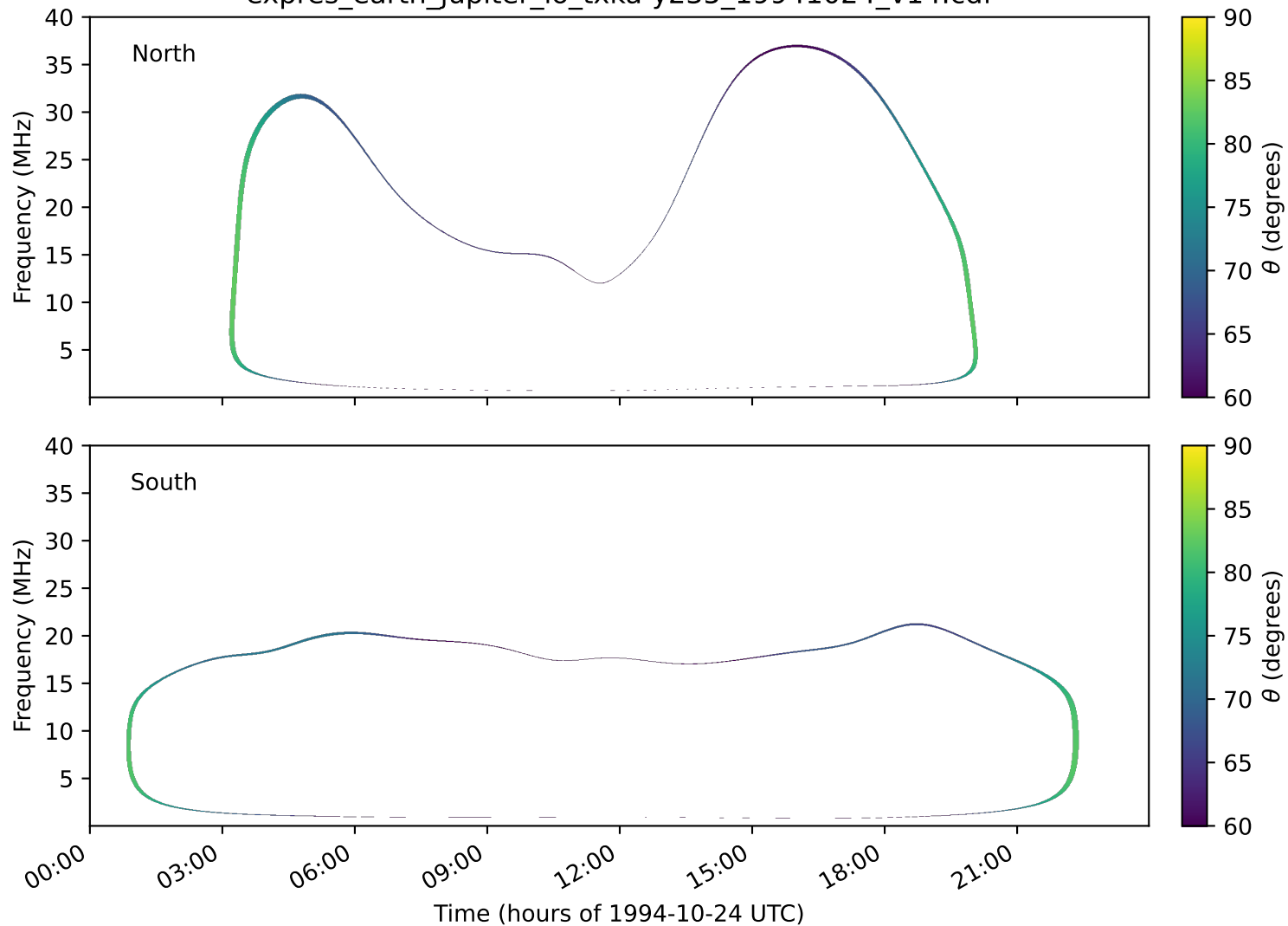
expres_earth_jupiter_io_txka-y235_19941024_v14.cdf
