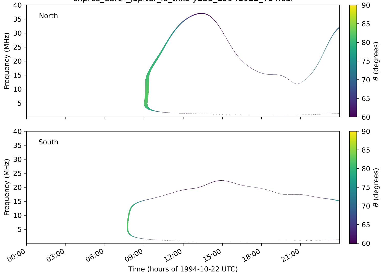
expres_earth_jupiter_io_txka-y235_19941022_v14.cdf
