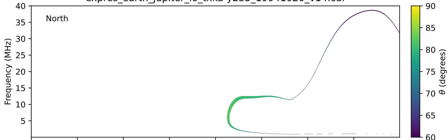
expres_earth_jupiter_io_txka-y235_19941020_v14.cdf
