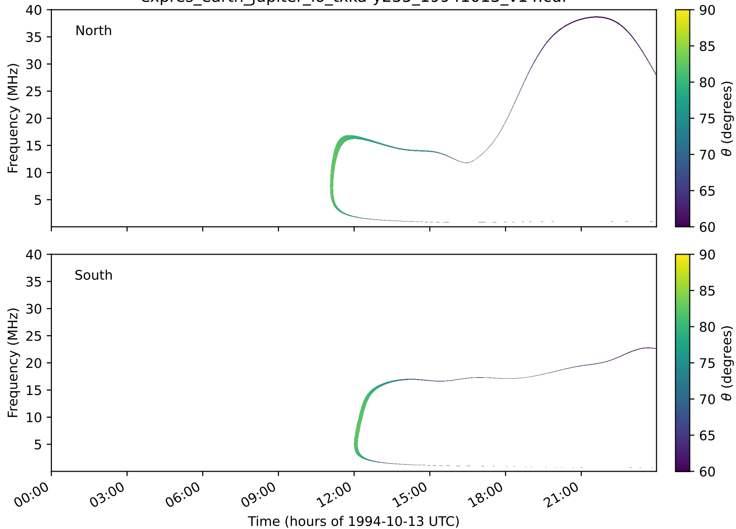
expres_earth_jupiter_io_txka-y235_19941013_v14.cdf
