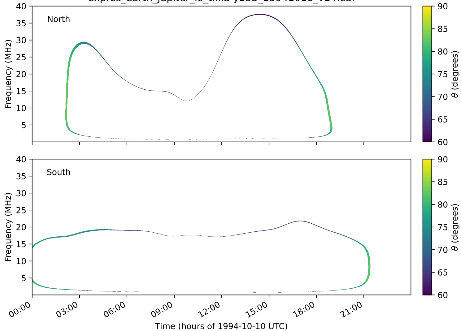
expres_earth_jupiter_io_txka-y235_19941010_v14.cdf
