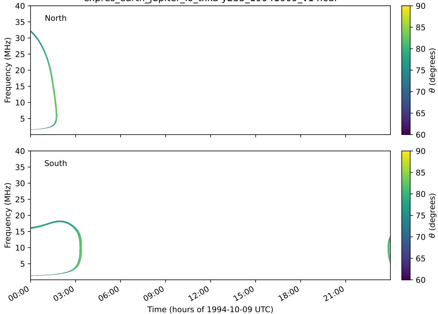
expres_earth_jupiter_io_txka-y235_19941009_v14.cdf
