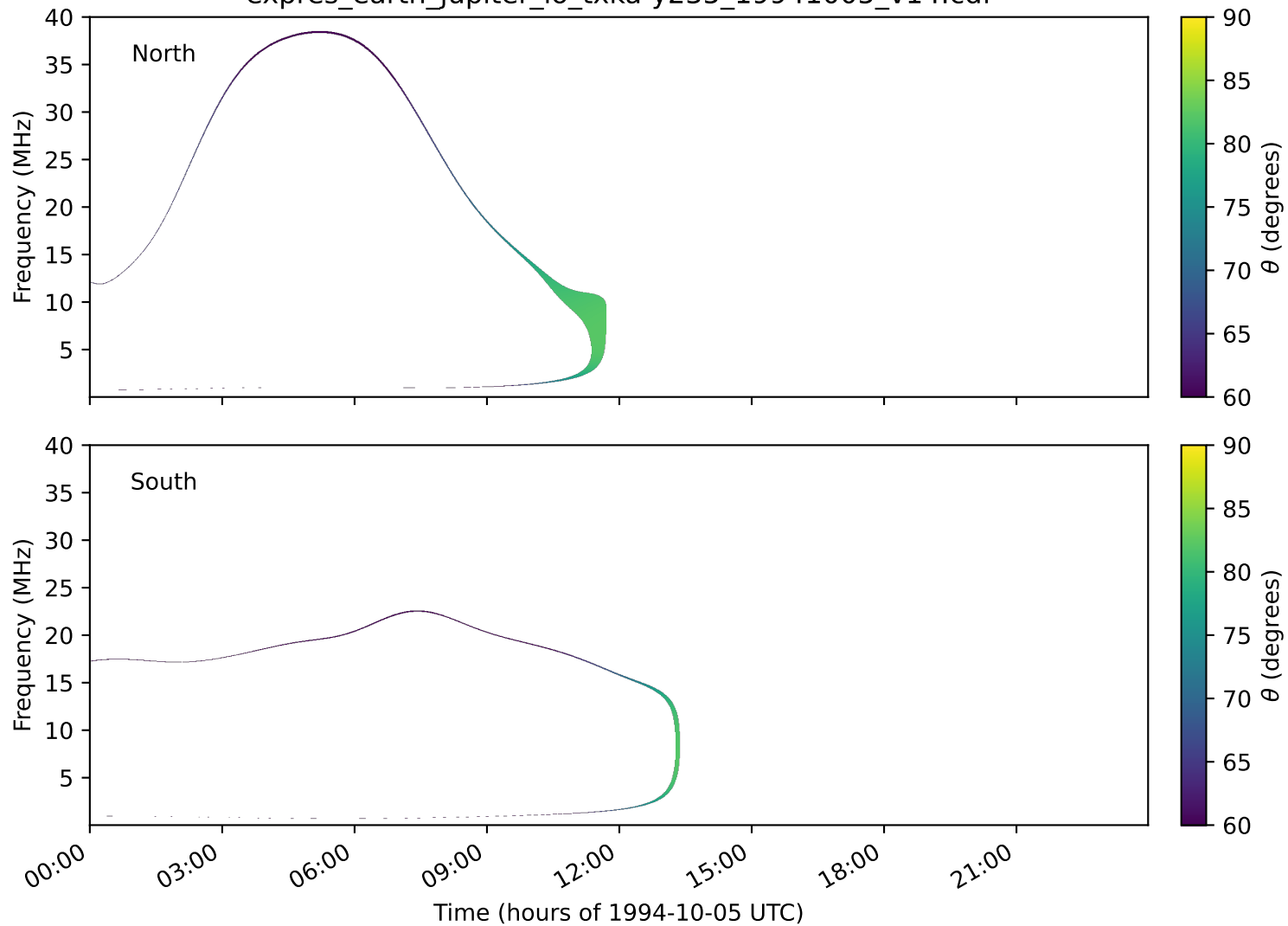
expres_earth_jupiter_io_txka-y235_19941005_v14.cdf
