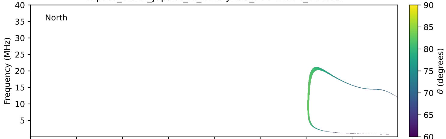
expres_earth_jupiter_io_txka-y235_19941004_v14.cdf
