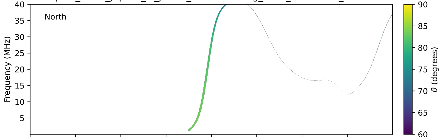
expres_earth_jupiter_io_jrm33_lossc-wid1deg_3kev_19941029_v11.cdf
