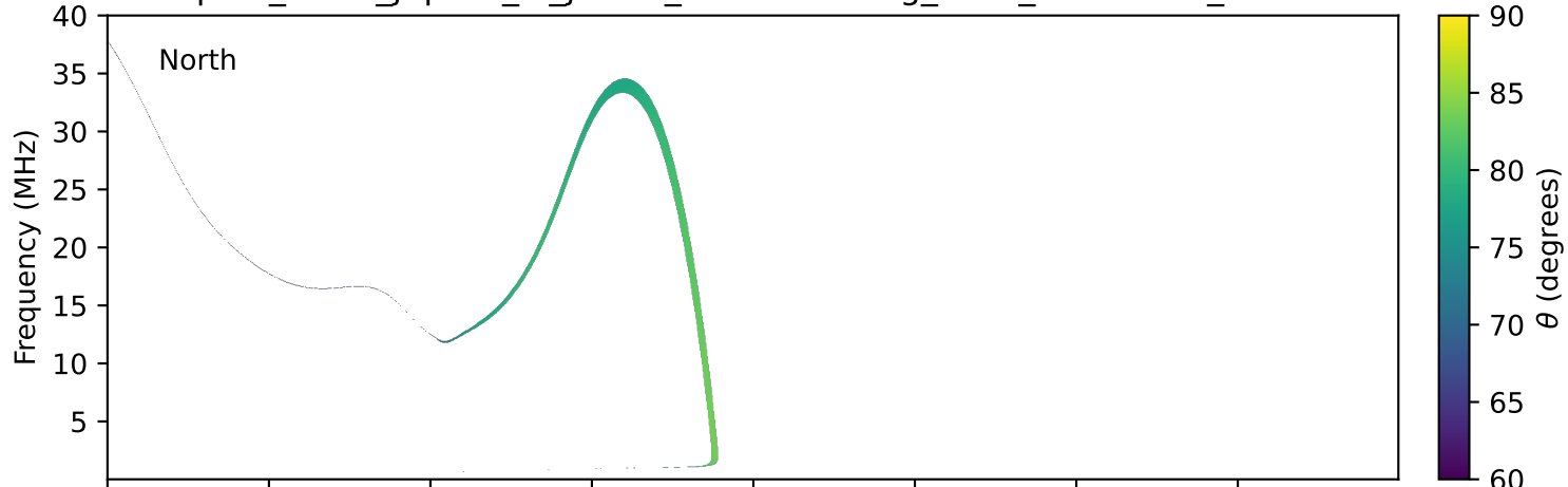
expres_earth_jupiter_io_jrm33_lossc-wid1deg_3kev_19941028_v11.cdf
