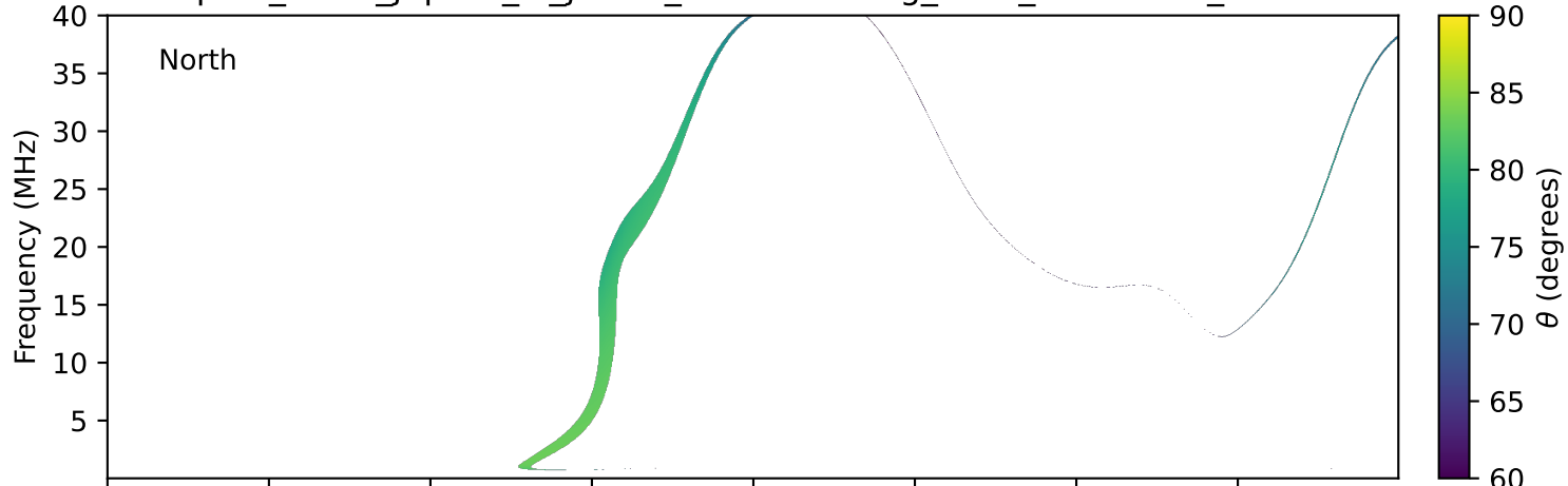
expres_earth_jupiter_io_jrm33_lossc-wid1deg_3kev_19941022_v11.cdf
