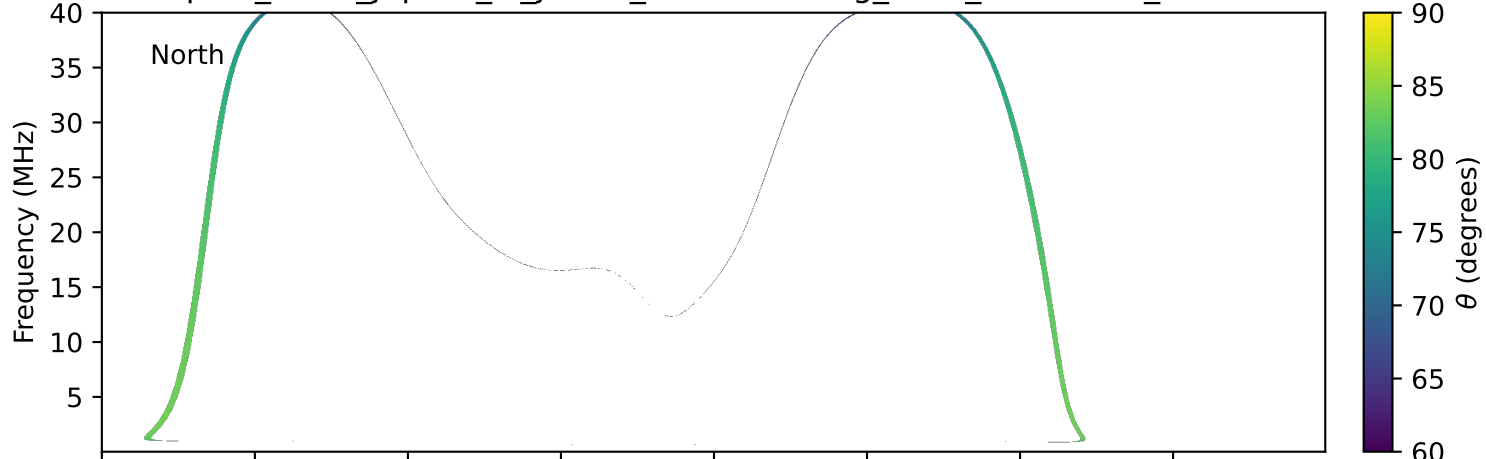
expres_earth_jupiter_io_jrm33_lossc-wid1deg_3kev_19941017_v11.cdf
