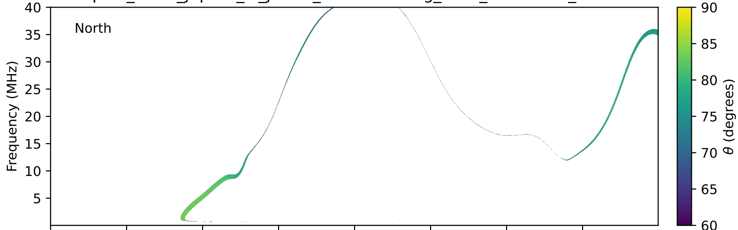
expres_earth_jupiter_io_jrm33_lossc-wid1deg_3kev_19941015_v11.cdf
