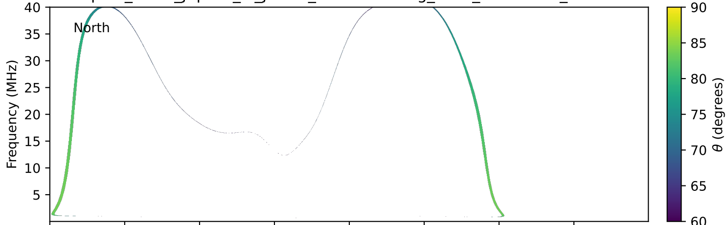
expres_earth_jupiter_io_jrm33_lossc-wid1deg_3kev_19941003_v11.cdf
