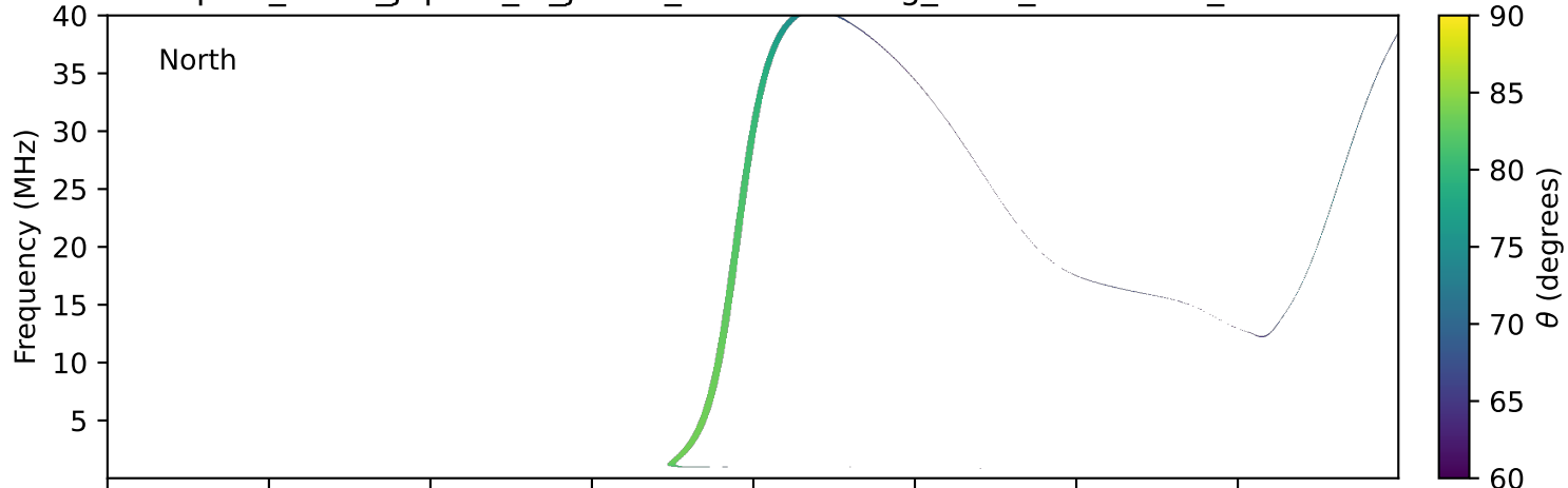
expres_earth_jupiter_io_jrm09_lossc-wid1deg_3kev_19941029_v11.cdf
