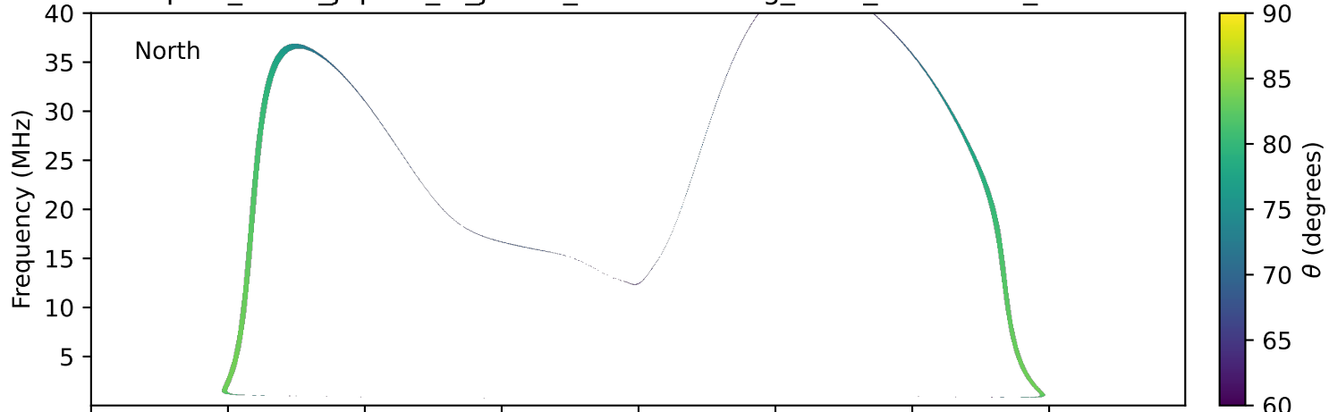
expres_earth_jupiter_io_jrm09_lossc-wid1deg_3kev_19941024_v11.cdf
