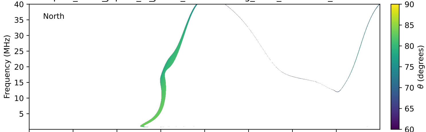
expres_earth_jupiter_io_jrm09_lossc-wid1deg_3kev_19941022_v11.cdf
