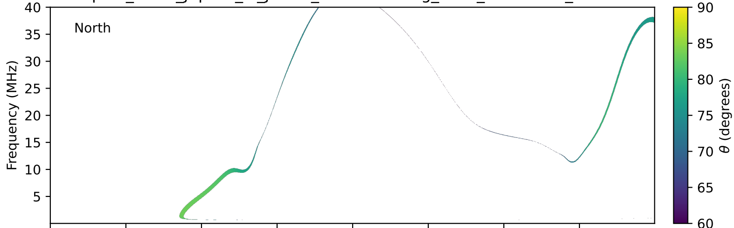
expres_earth_jupiter_io_jrm09_lossc-wid1deg_3kev_19941015_v11.cdf
