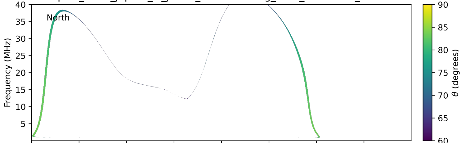
expres_earth_jupiter_io_jrm09_lossc-wid1deg_3kev_19941003_v11.cdf
