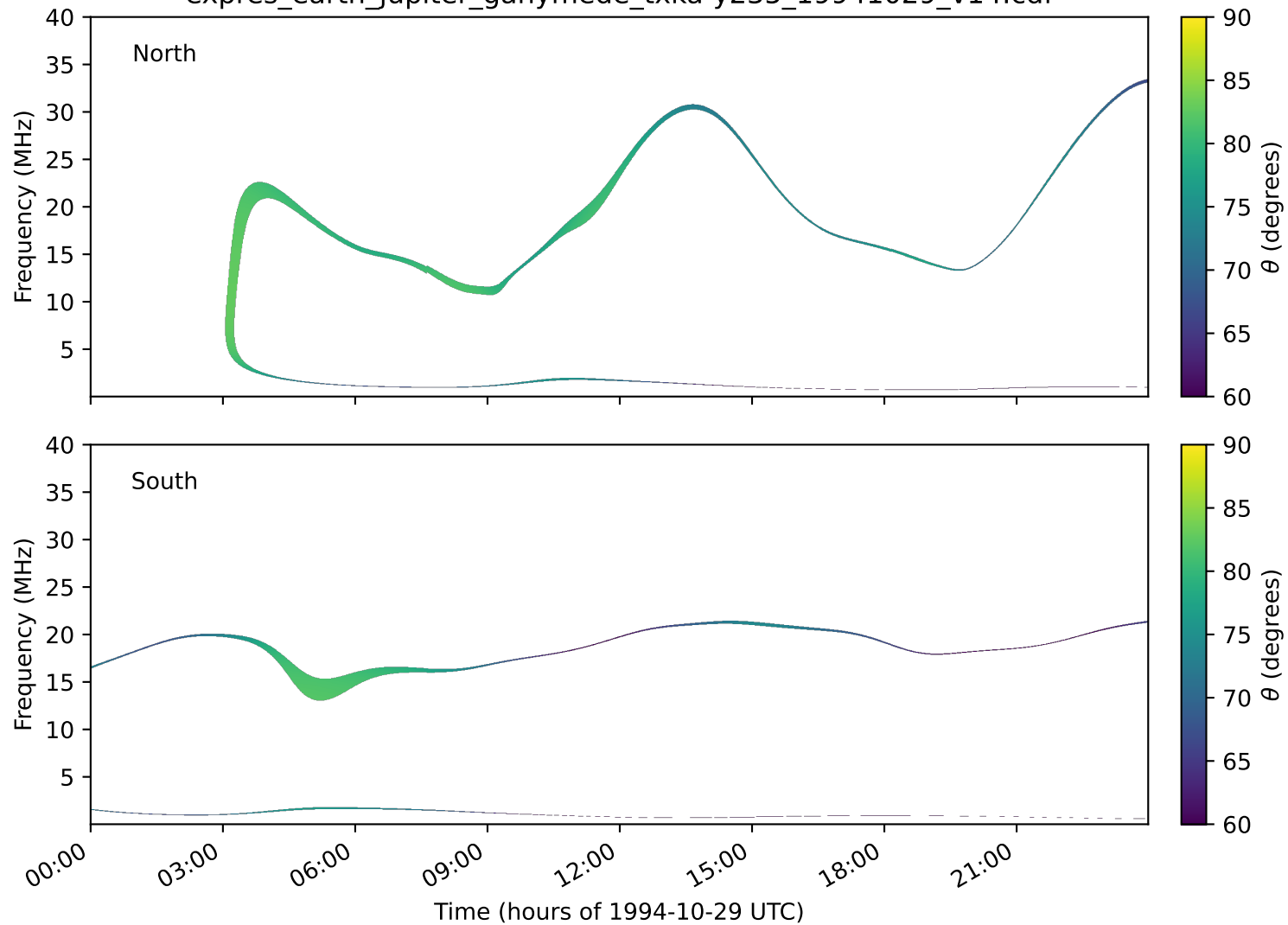
expres_earth_jupiter_ganymede_txka-y235_19941029_v14.cdf
