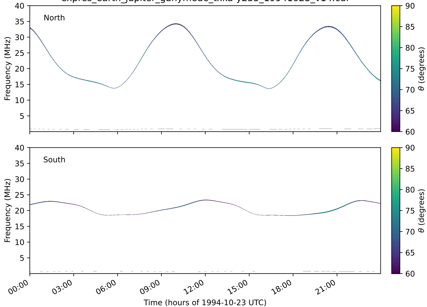
expres_earth_jupiter_ganymede_txka-y235_19941023_v14.cdf
