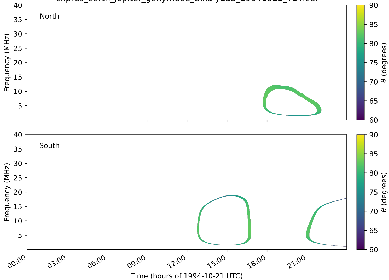
expres_earth_jupiter_ganymede_txka-y235_19941021_v14.cdf
