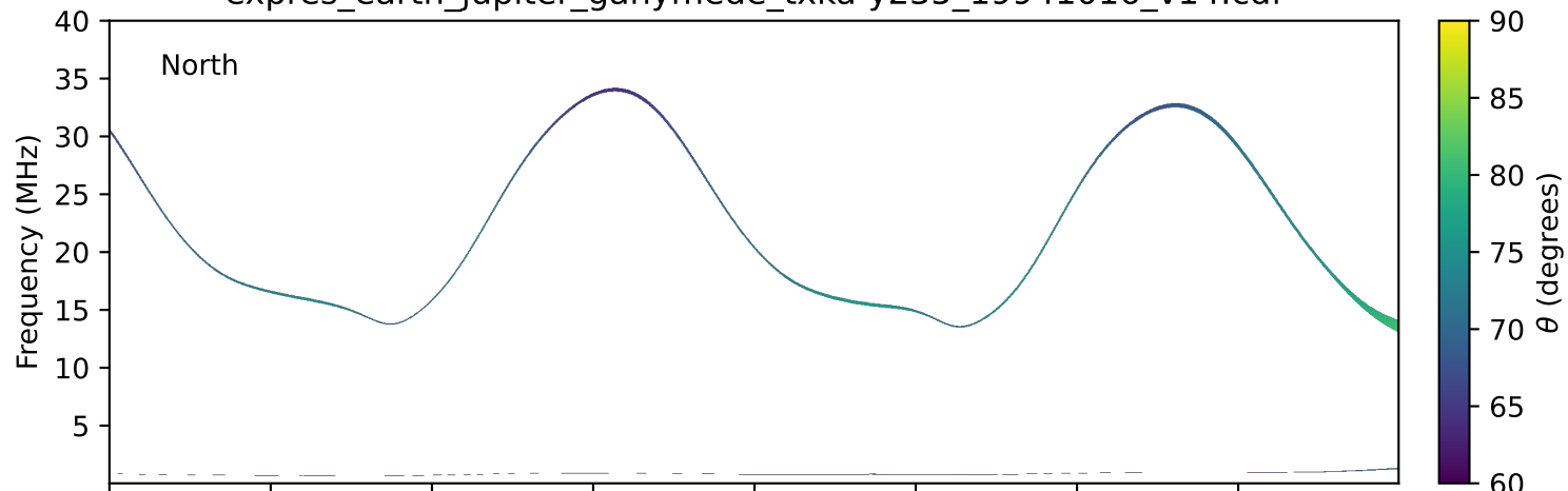
expres_earth_jupiter_ganymede_txka-y235_19941016_v14.cdf
