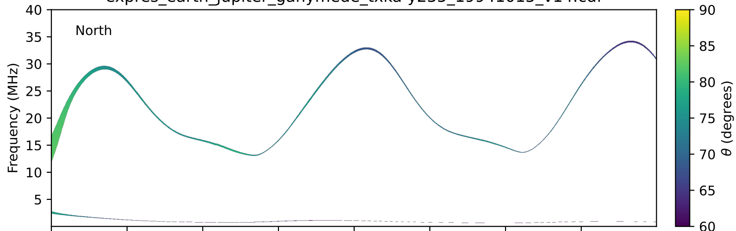
expres_earth_jupiter_ganymede_txka-y235_19941015_v14.cdf
