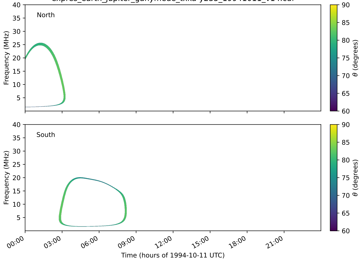
expres_earth_jupiter_ganymede_txka-y235_19941011_v14.cdf
