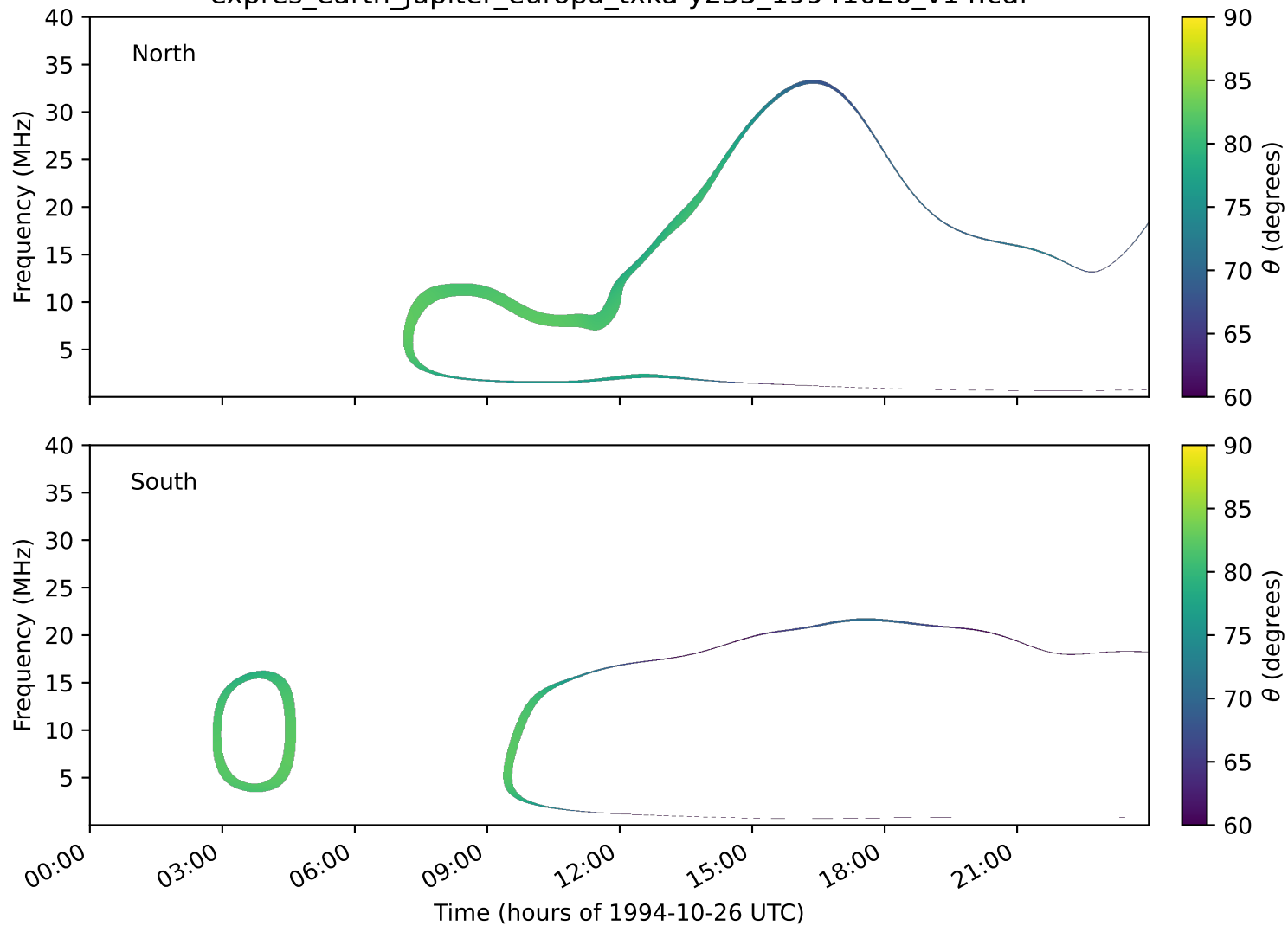
expres_earth_jupiter_europa_txka-y235_19941026_v14.cdf
