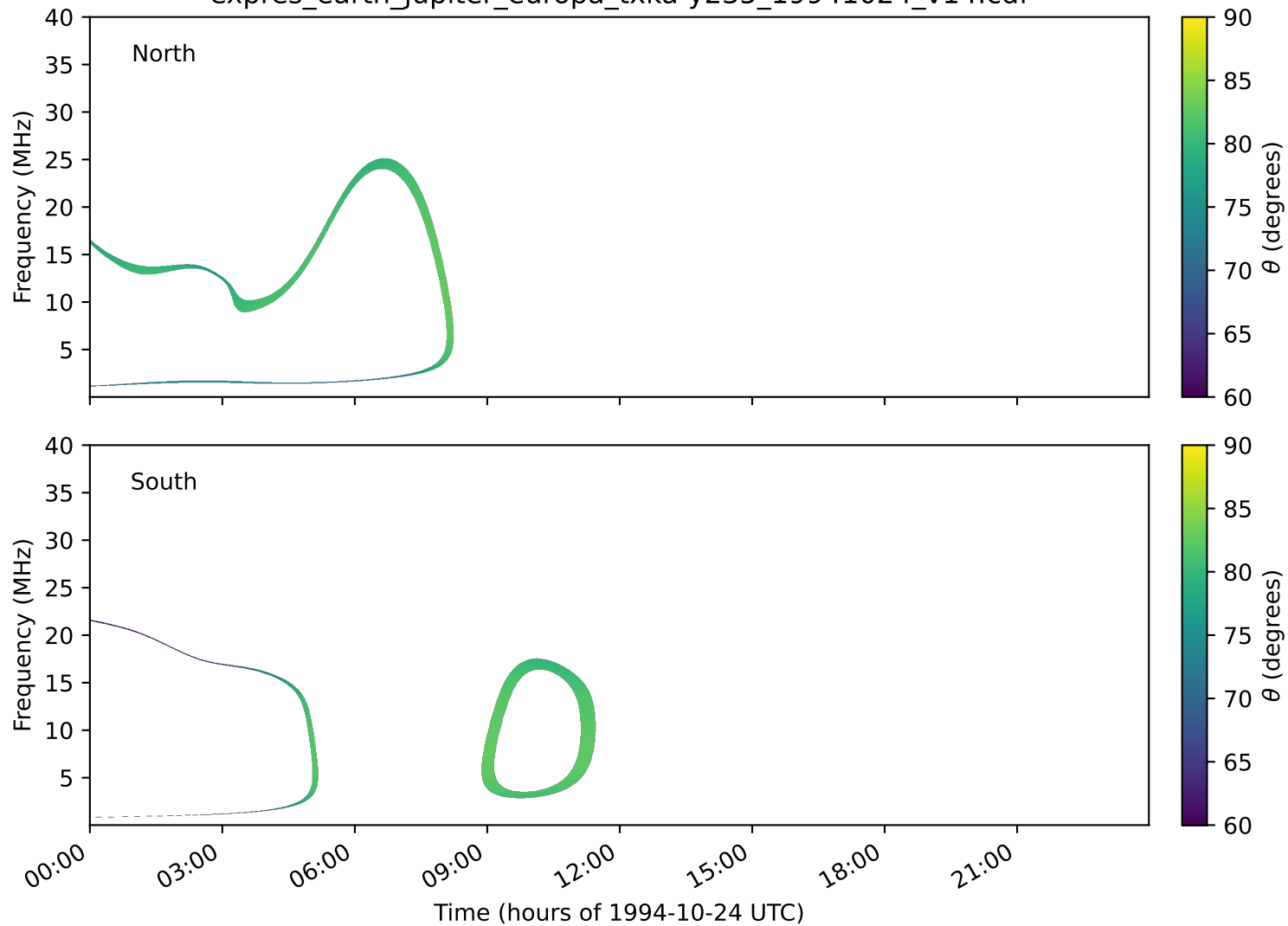
expres_earth_jupiter_europa_txka-y235_19941024_v14.cdf
